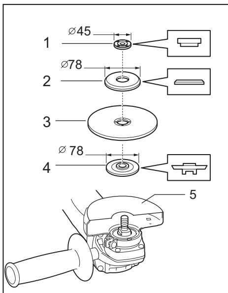
► 1. Lock nut 2. Outer flange 78 3. Abrasive cut-off wheel/diamond wheel 4. Inner flange 78 5. Wheel guard for abrasive cut-off wheel/diamond wheel
